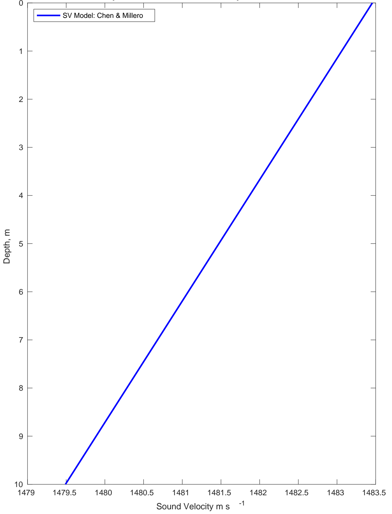
Sound Velocity Profile for DOD AO on 02-May-2024 00:00:00
